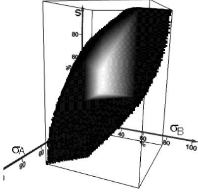
Figure 1: Viability domain D for the problem of language coexistence. The bounding box is the set of desirable states. Evolution starting in D can stay within forever.
