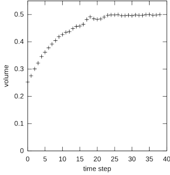
Figure 3: Evolution of the volume of the capture basin with time horizon. Convergence to 0.5 occurs around time step 25. (In this experiment the splitting direction in refined node is selected randomly, so the convergence is not monotonous)
