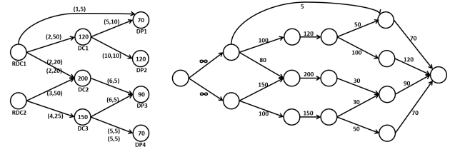
Figure 1: (Left) The tuple on a link represents the maximum number of trips and vehicle capacity respectively. The number on a DC is its holding capacity, and the number on a demand point is the requested quantity. (Right) The flow network constructed from the assignment, with max flow of 215, providing 61.43% service level.
