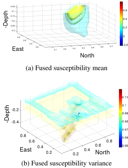
Figure 9: Joint inversion results for susceptibility with fusion model that includes gravity and magnetic data of the dipping body.
