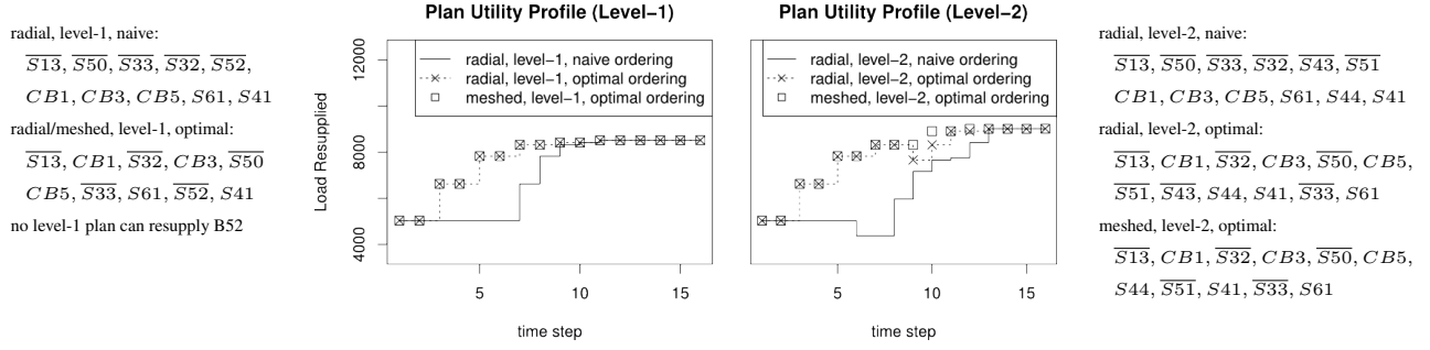
Figure 2: Load supplied by level-1 plans (left) and level-2 plans (right) as a function of plan step, under different operation orderings (naïve vs optimal) and network topology (radial vs meshed). “Naïve” order has all openings first and then all closings. Faults are on B14, B51, and B33 of Figure 1. In the plan descriptions, S means “close S ” and \bar{S} means “open S ”. Observe that the level-1 plans (left) are shorter but resupply less load than the level-2 plans (right), that meshed topologies reduce level-2 plan length and avoid the service interruptions (curve drops) observed with radial topologies, and that naive operation ordering yields poor utility (the area under the curve is smaller).
