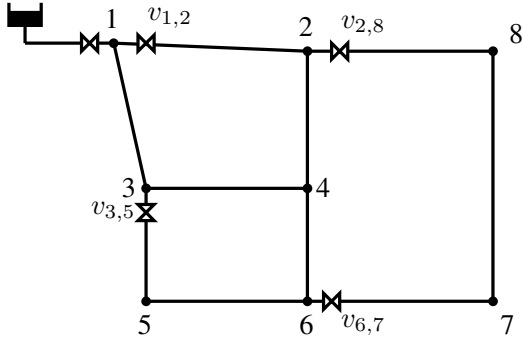
Figure 2: A network with redundant valves
