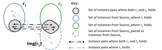
Figure 2: Comparing linked instances from two ontologies
