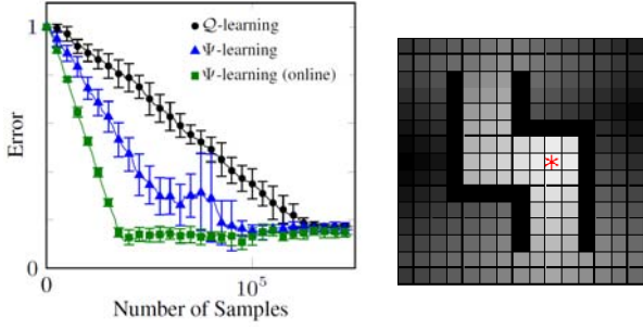
Figure 3: Results from the Gridworld problem. (left) Evolution of the mean error in (9) averaged over 10 trials with error bars indicating the s.d. (right) Optimal value function (white low expected cost - black high expected cost) of the problem. Obstacles are black and the target state is indicated by *.
