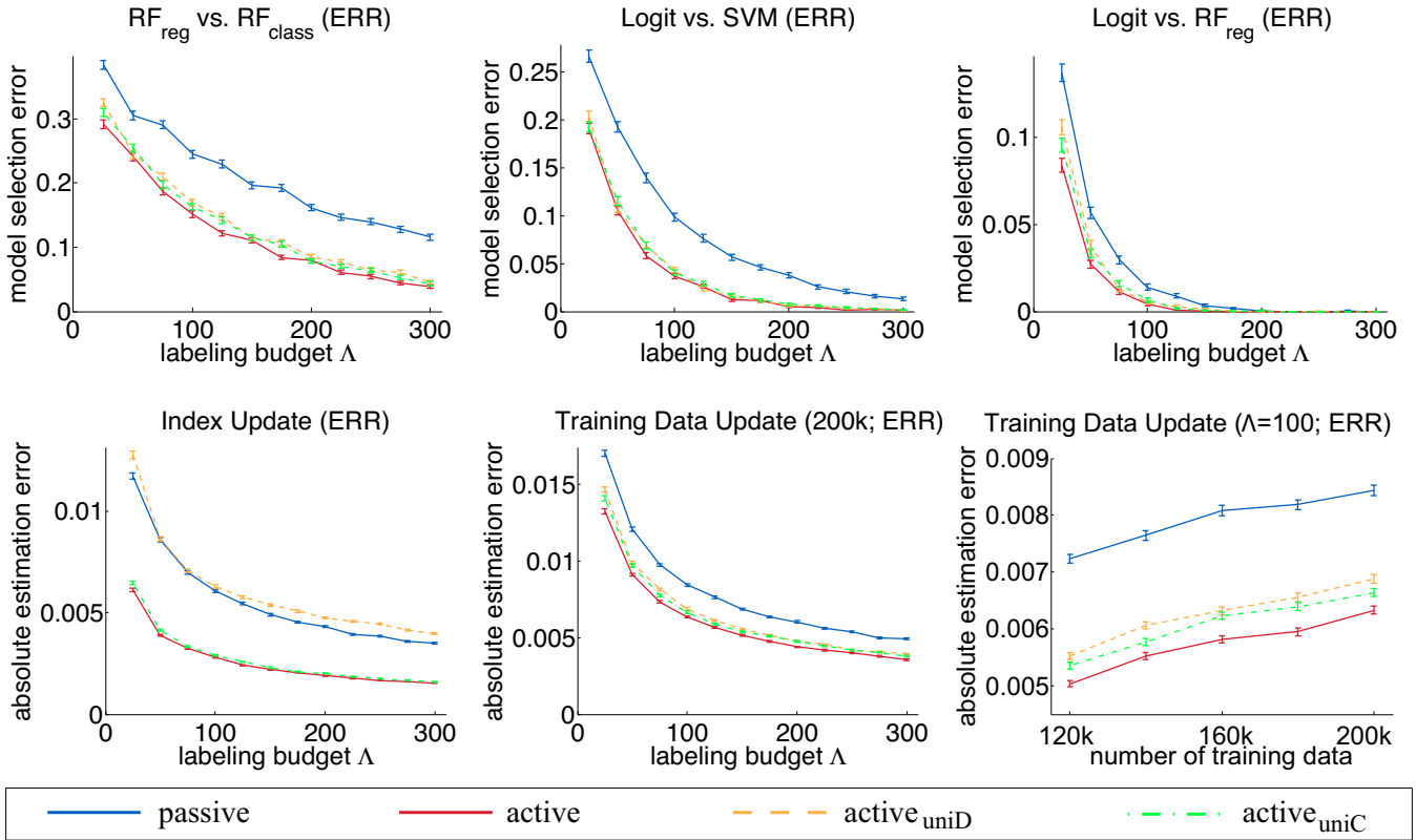
Figure 1: Top row: Model selection error over \Delta when comparing Random Forest regression vs. classification (left), and Ordered Logit vs. Ranking SVM (center) or Random Forest regression (right). Bottom row: Absolute estimation error over \Delta for a simulated index update (left). Absolute estimation error comparing ranking functions trained on 100,000 vs. 200,000 query-document pairs over \Delta (center), and over training set size of second model at \Delta = 100 (right). Error bars indicate the standard error.
