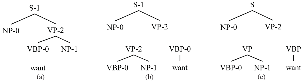
Figure 2: Example three-level backoff.. (a) Example SR-TSG rule. (b) SR-CFG rules of (a). (c) RU-CFG rules of (b).
