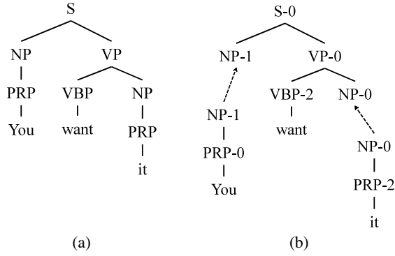
Figure 1: (a) Example parse tree. (b) Example SR-TSG derivation of (a). The refinement annotation is hyphenated with a nonterminal symbol.
