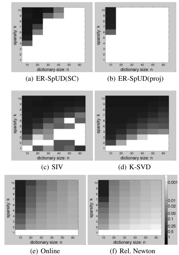
Figure 1: Mean relative errors over 10 trials, with varying support k (y-axis, increase from bottom to top) and basis size n (x-axis, increase from left to right). Here, p = 5n \log_e n . Our algorithm using a column of Y as r (ER-SpUD(SC)), SIV [Gottlieb and Neylon, 2010], K-SVD [Aharon et al. , 2006], online dictionary learning [Mairal et al. , 2009], and the relative Newton method for source separation [Zibulevsky, 2003].
