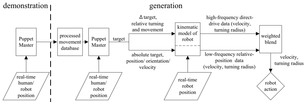
Figure 3. The algorithm data-flow and processing, and how Puppet Master connects to the real-time robot data.
