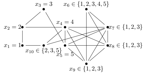
Figure 1: A graph coloring problem where we can exploit additional symmetries.
