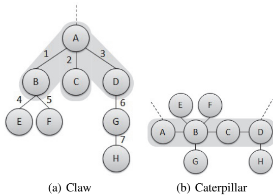
Figure 1: Self-Reinforcing Structures
