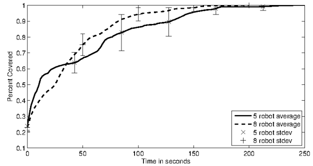
Figure 1: Average percent of the environment covered over time for five and eight robots (ten runs each). Error bars show standard deviation at that time point.
