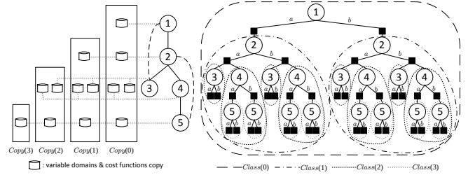
Figure 1: Left: The pseudo-tree of a DCOP. Right: Search tree ( a/b domains), subproblems and classes of subproblems. and FDAC asynchronously in all subproblems during search by utilizing additional copies of variable domains and cost functions in each agent. We use an agent classing scheme based on the position of an agent in the problem structure. The scheme governs the required number of copies of variable domains and cost functions in an agent. With extra copies of variable domains and cost functions, the consistency enforcement in different subproblems can be performed asynchronously. However, it is unnecessary to maintain a copy for each subproblem for space efficiency. For example, Figure 1 Right illustrates the search tree, subproblems and classes of subproblems of a DCOP with 5 agents and there are four classes of subproblems. Each agent holds a variable domains and cost functions copy for each class of subproblem (Figure 1 Left). Therefore, the consistency enforcement in the four classes of subproblems can be performed asynchronously. In the following, we outline the issues and solutions used in maintaining AC and FDAC in BnB-ADOPT + .
