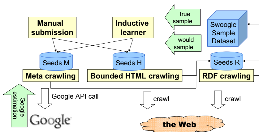
Fig. 2. The Swoogle system uses an adaptive Semantic Web harvesting framework with three different kinds of crawlers
