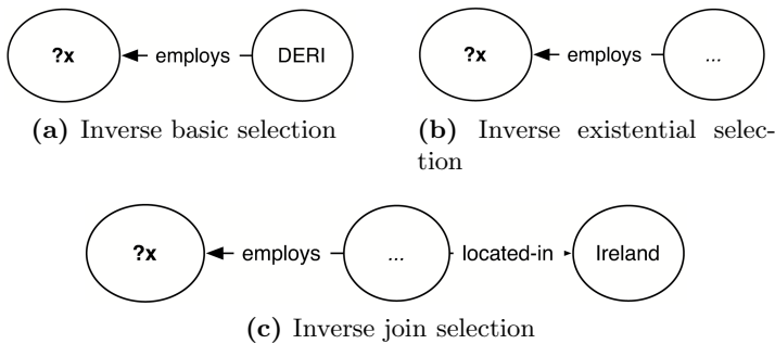
Fig. 4. Inverse operators
