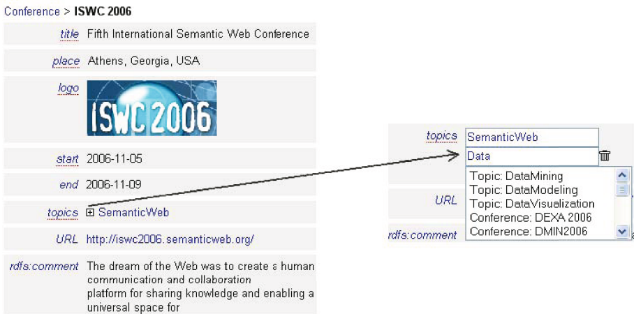
Fig. 3. OntoWiki instance display with statement edit buttons (left). Statement editor with interactive search for predefined individuals based on AJAX technology (right).
