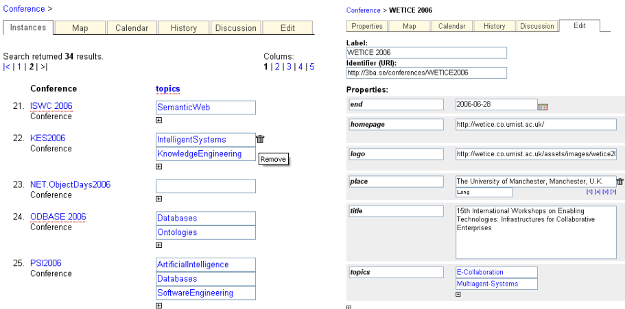
Fig. 4. Editing of a property's values at many instances at once (left). Dynamically generated form combining different widgets based on an OWL class definition (right).
