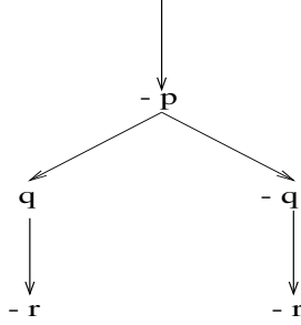
Figure 1: A quantifier tree.
