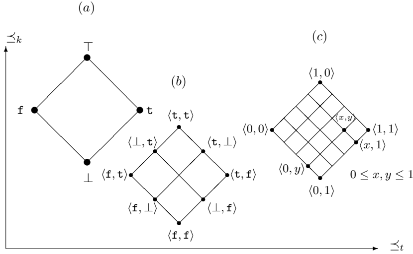
Figure 1: Bilattices. (a) \mathcal{F}\mathcal{O}\mathcal{U}\mathcal{R} , (b) \{\mathbf{f}, \bot, \mathbf{t}\} \odot \{\mathbf{f}, \bot, \mathbf{t}\} and (c) \mathcal{K}([0, 1]) .
