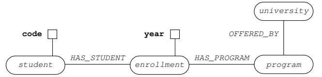
Figure 3: Diagrammatic representation of the students ontology
