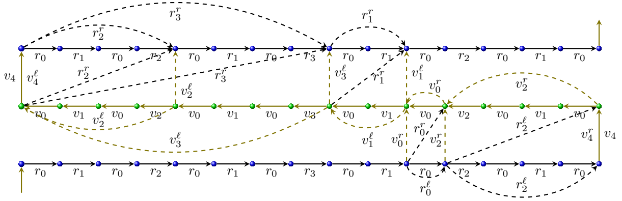
Figure 5: Connecting the corresponding elements of r -chains using linear RIAs
