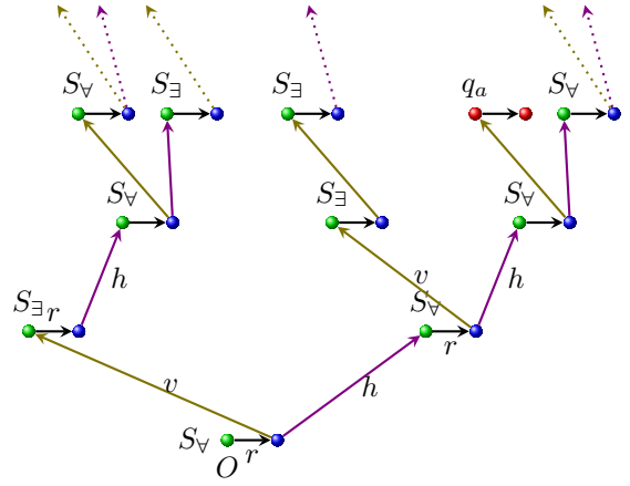
Figure 4: Encoding a computation of an ATM
