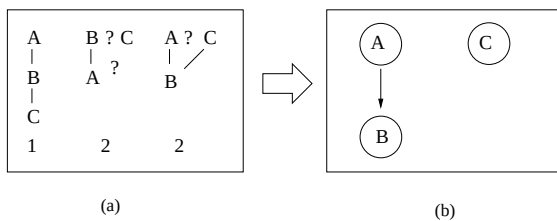
Figure 1: An incomplete weighted profile and its majority graph.
