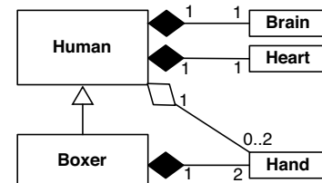
Figure 1: UML diagram with part-whole relations.
