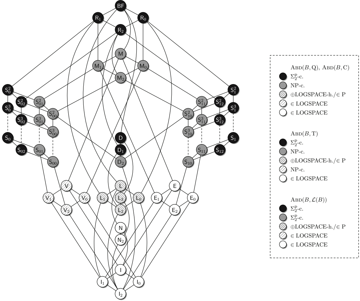
Fig. 1. Post's lattice showing the complexity of the abduction problem \text{ABD}(B, \mathcal{M}) for all sets B of Boolean functions and considered restrictions \mathcal{M} of the manifestations.
