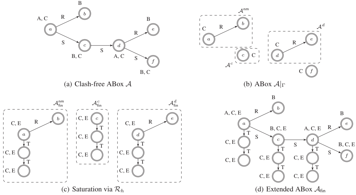
Figure 3: Completeness of the \mathcal{ALCHIQ} \Omega^a -algorithm
