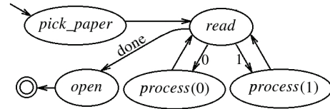
Figure 7: Axioms and a solution plan for safe
