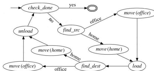
Figure 1: An example plan for the logistic problem
