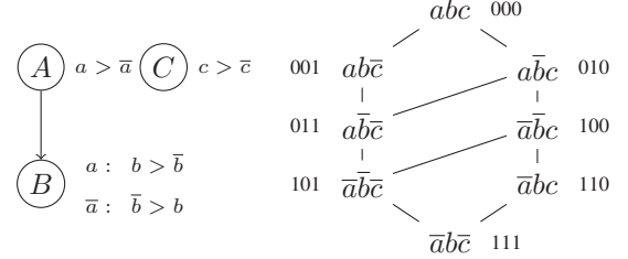
Figure 3: An acyclic CP-net and its solution ordering.
