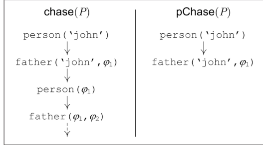
Figure 1: \text{chase}(P) vs \text{pChase}(P) w.r.t. Example 3.2
