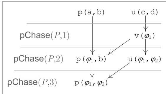
Figure 2: Snapshot of pChase(P, 3) w.r.t. Example 4.11
