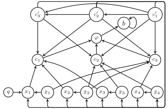
Figure 3: Illustration of the AF F_{\varphi, x_1} for \varphi = (x_1 \vee x_2 \vee x_3) \wedge (\neg x_2 \vee \neg x_3 \vee \neg x_4) \wedge (\neg x_1 \vee \neg x_2 \vee x_4) .
