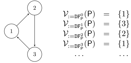
Figure 3: A 3-cycle attack graph, and the first four elements of the stream V := DF_P^\omega generated at the model whose valuation is V(P) = \{1\} . The stream cycles every three steps.
