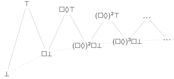
Figure 5: Decomposability of the stream := \neg \Diamond \perp^\omega .
