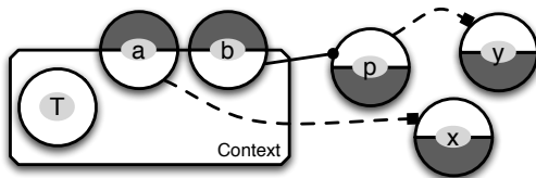
Figure 10: Combining N and C (Examples 13 and 14).
