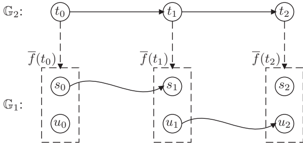
Figure 2: A transformation that is P 1↓ but not P 2↓ .
