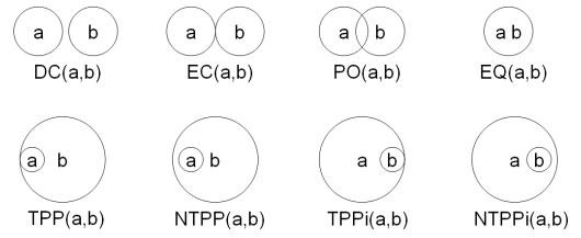
Figure 3: RCC8 base relations.
