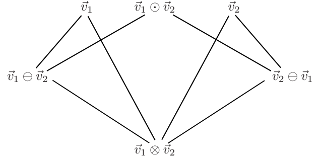
Figure 1: Hasse diagram showing the ordering (relative to \leq ) of the different valuation pairs resulting from applying the operators \otimes , \ominus and \odot to \vec{v}_1 and \vec{v}_2 .
