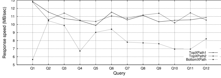
Fig. 2. Query response speed (averaged over the document series)
