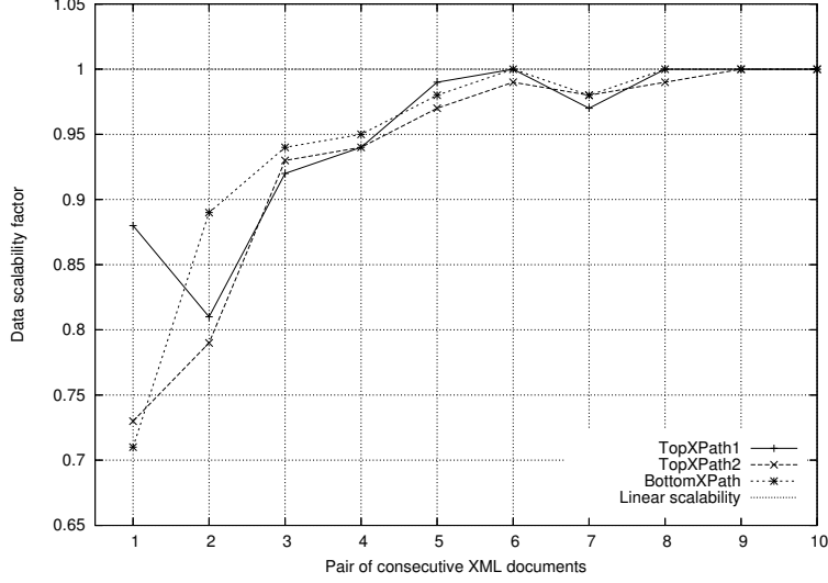
Fig. 3. Data scalability factors (averaged over the benchmark set)
