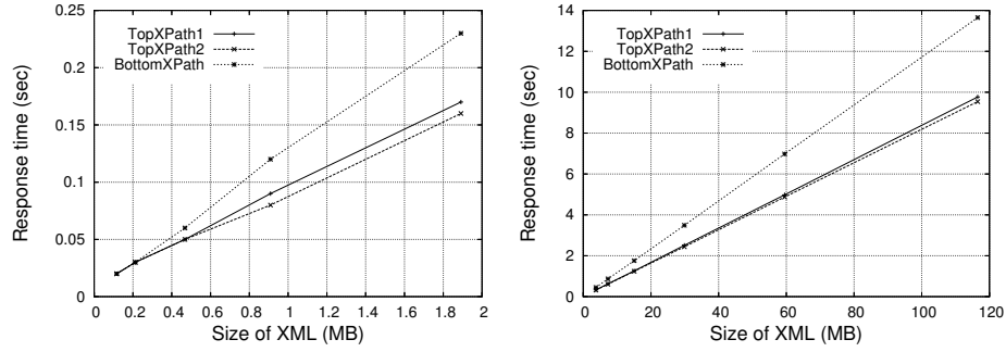
Fig. 1. Query response time (averaged over the benchmark set)
