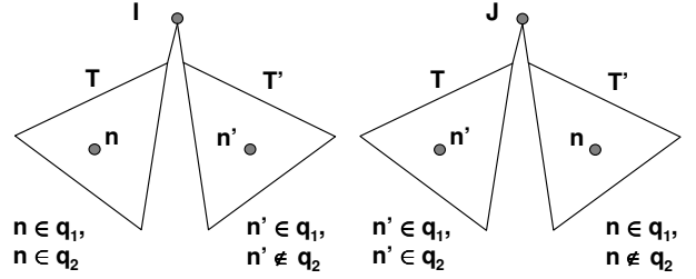
Figure 3: Counterexample pair of instances (I, J) .
