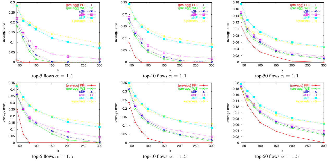
Figure 2: Pareto \alpha = 1.1 and \alpha = 1.5 , estimating subset consisting of top-5, top-10, and top-50 flows.
