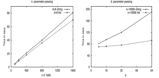
Figure 3: Comparing UDF parameter passing style.
