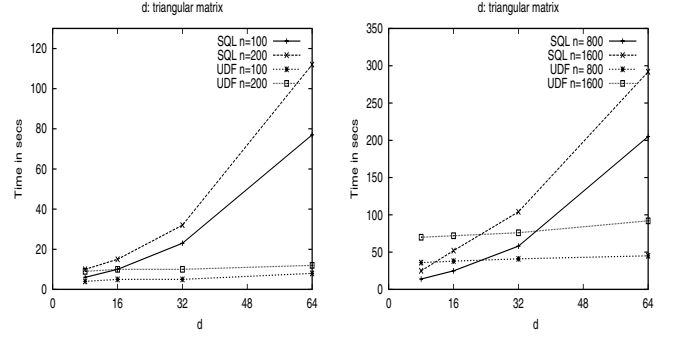
Figure 2: SQL vs. aggregate UDF varying d .
