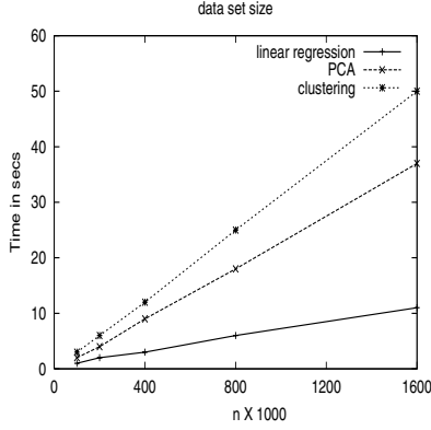
Figure 6: Scalar UDFs to score: Time varying n .
