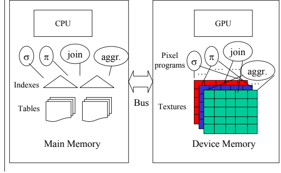
Figure 1: Illustration of GPU Query Co-Processing
