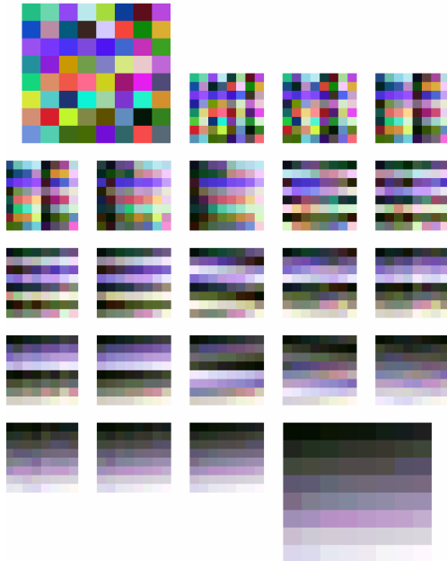
Figure 2: Illustration of GPUSort
