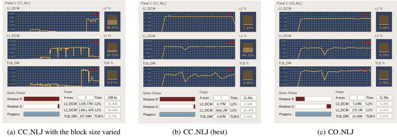
Figure 3: Screen shots: CO_NLJ and CC_NLJ on P4
