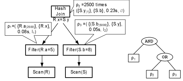
Figure 2: Execution plan and AND/OR request tree.
