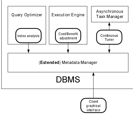
Figure 1: Continuous Tuning Architecture in a DBMS.
