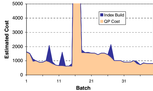
Figure 4: Online schedule for a complex TPC-H workload.
