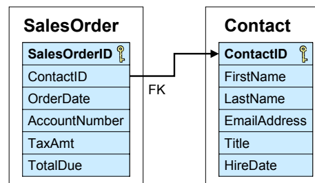
Figure 1: Sample relational schema
