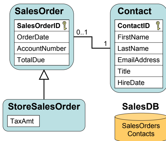
Figure 2: Sample EDM schema
