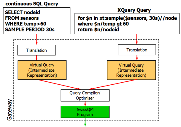
Figure 2: SwissQM Language Handlers
