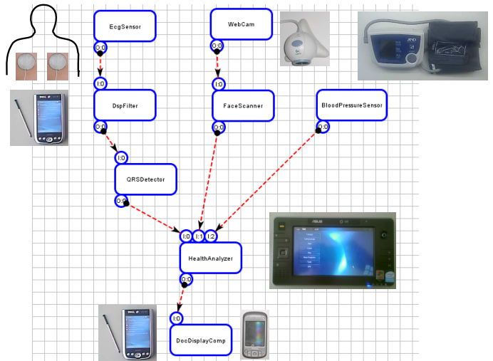
Figure 2: Demo Process
