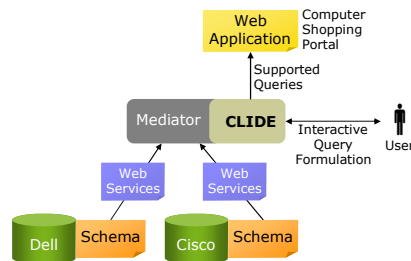
Figure 1: Service-Oriented Architecture
