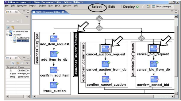
Figure 2: Selection from a BPEL specification.
