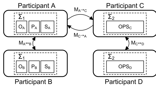
Figure 2: A CDSS for four bioinformatics sources. Participants A and B share a common schema, as do participants C and D, so mappings M_{A \leftrightarrow B} and M_{C \leftrightarrow D} are identity mappings. The mapping M_{A \rightarrow C} translates the three tables of schema \Sigma_1 into the single table of \Sigma_2 , and M_{C \rightarrow A} does the inverse.
