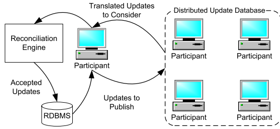
Figure 1: An overview of the architecture of a CDSS. Here the published transactions are stored in a peer-to-peer distributed database, though one can also use other methods to store the published updates.
