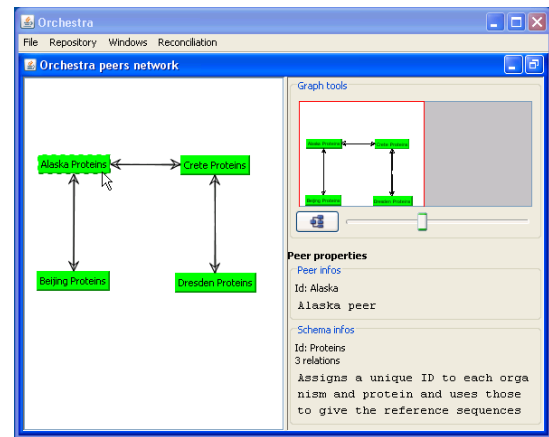
Figure 3: The mapping viewer of the Java-based GUI.
