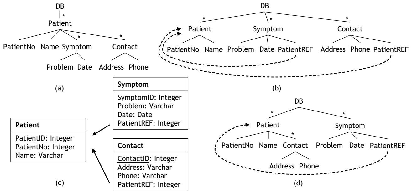
Figure 1: Databases Schemas
