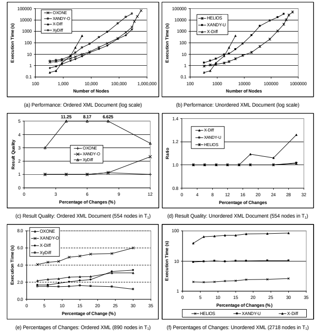
Figure 4: Performance results.
