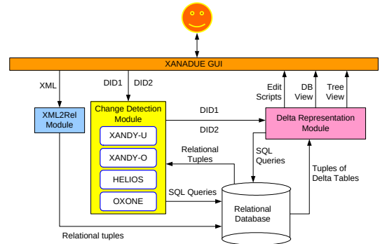
Figure 1: System Architecture of XANADUE.
