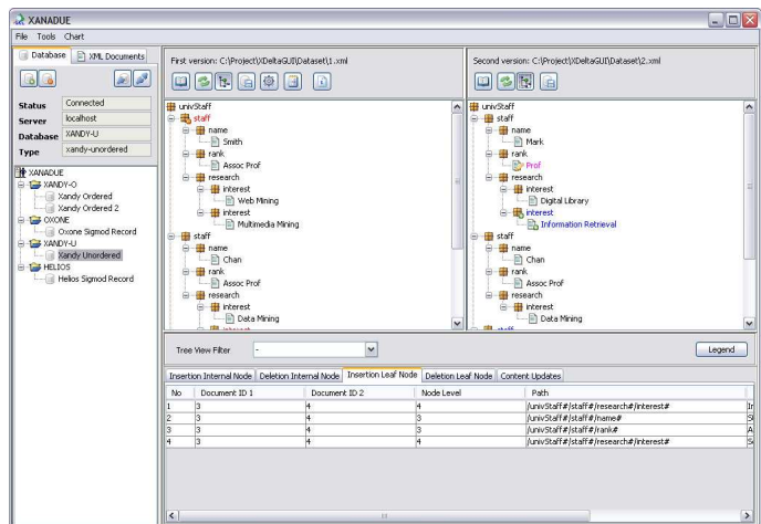
Figure 2: XANADUE GUI.
