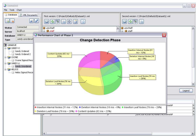
Figure 3: Performance visualization.
